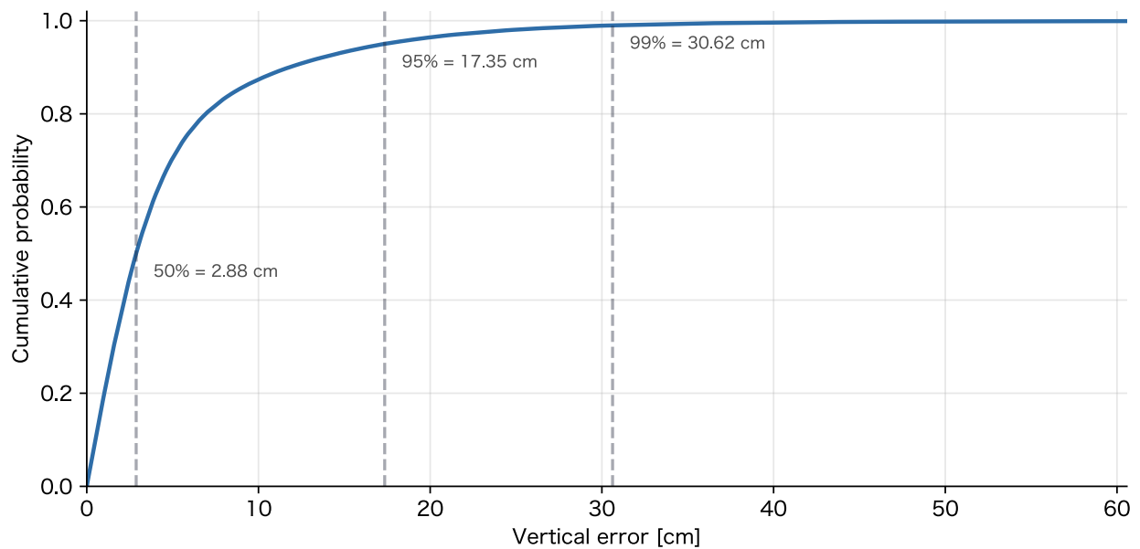
Figure 3: Cumulative distribution of vertical error (epochs pooled over qualified stations).
