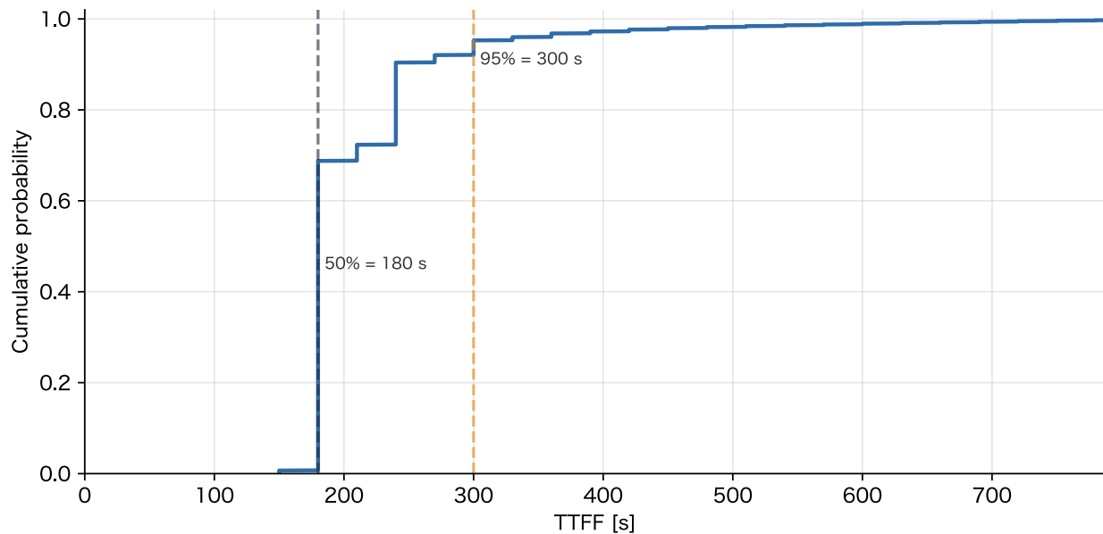
Figure 4: Cumulative distribution of TTFF (15-min reset, reset windows pooled nationwide over the period).
